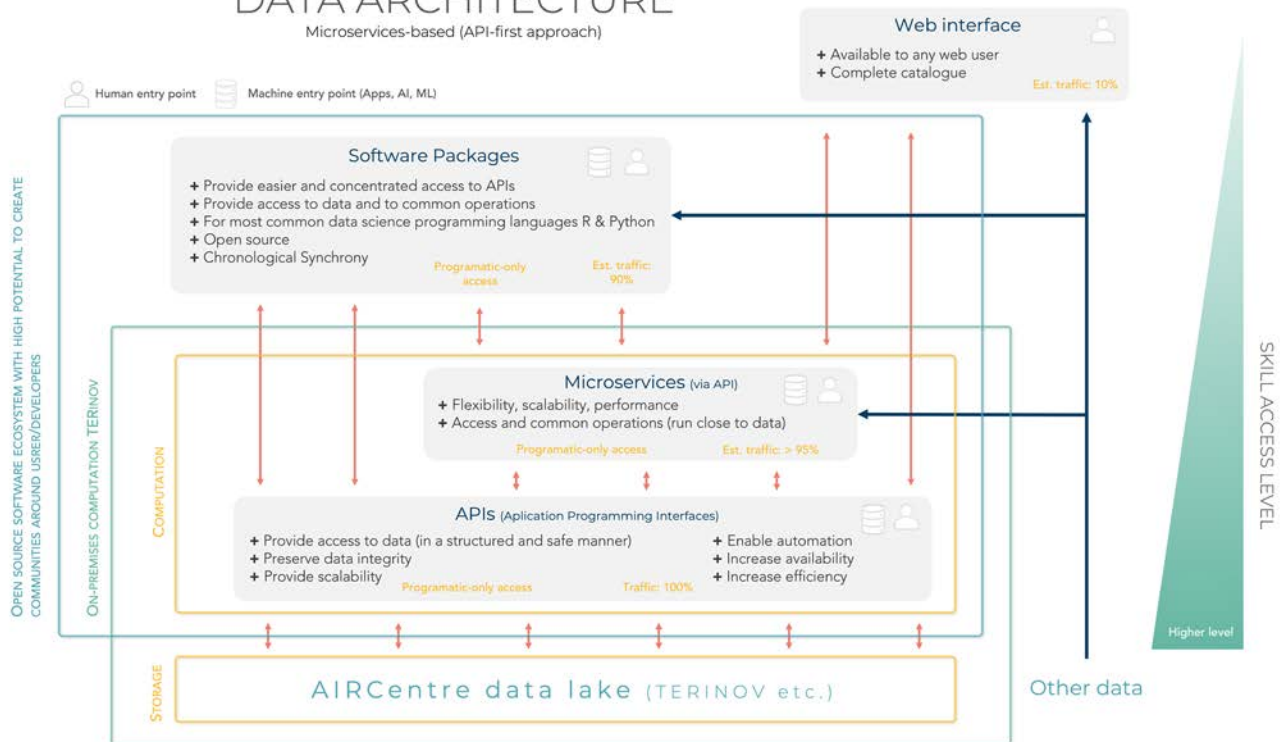
Figure 28 - System conception and architecture for data management at the AIR Data Center
